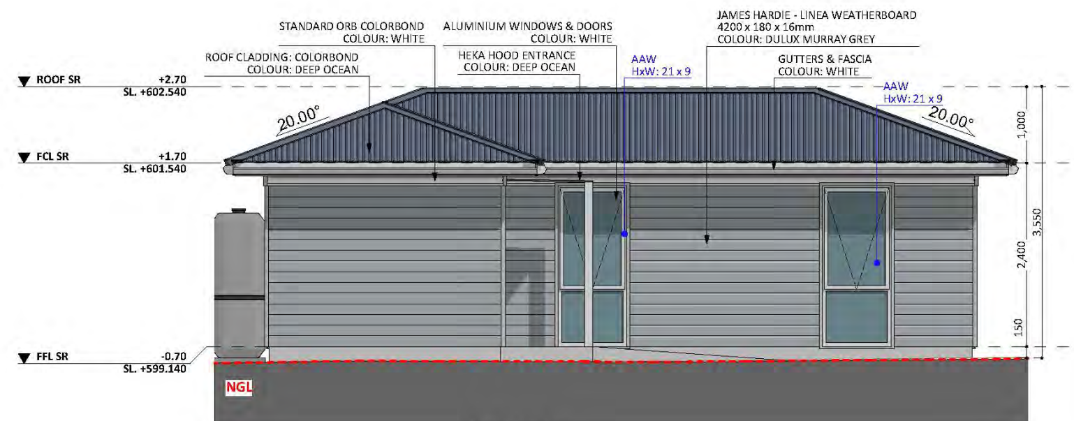
SOUTH ELEV.
