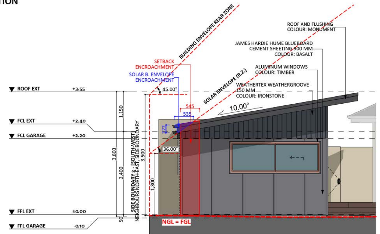
SOUTH-EAST ELEVATION
