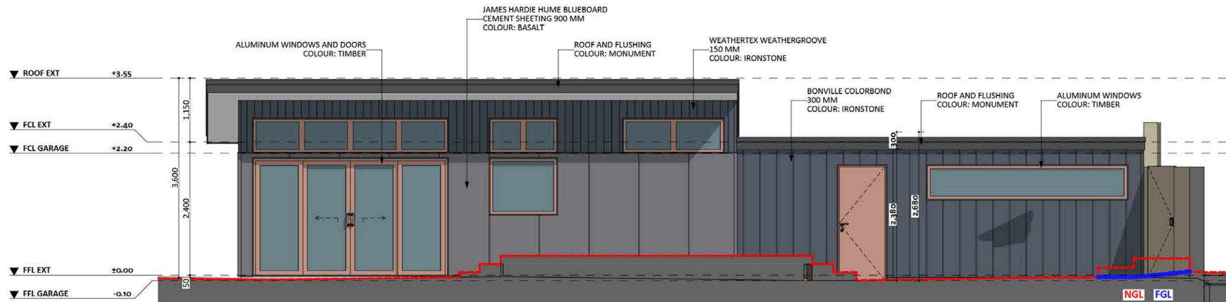
NORTH-EAST ELEVATION
