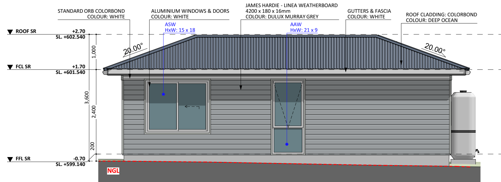
NORTH ELEV.
