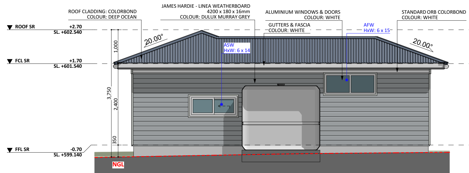
WEST ELEV.
