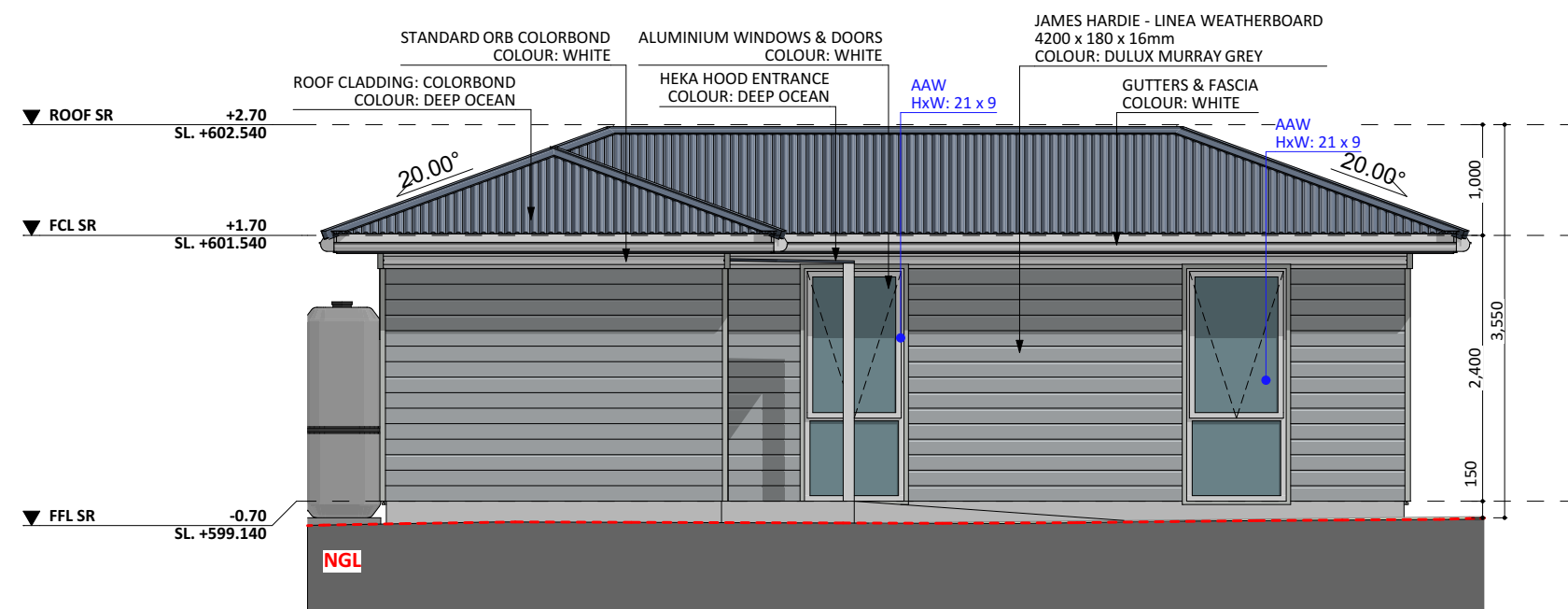
SOUTH ELEV.
