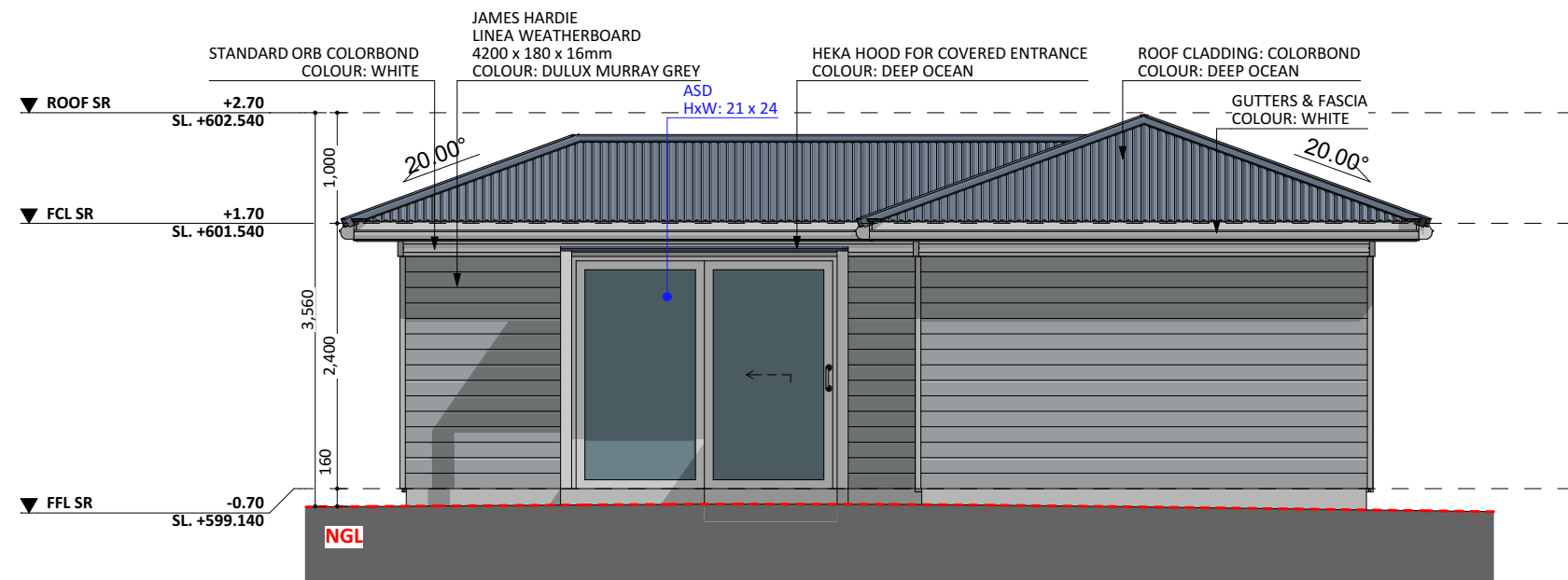
EAST ELEV.
